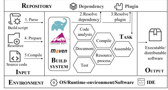
Figure 1: Build workflow
